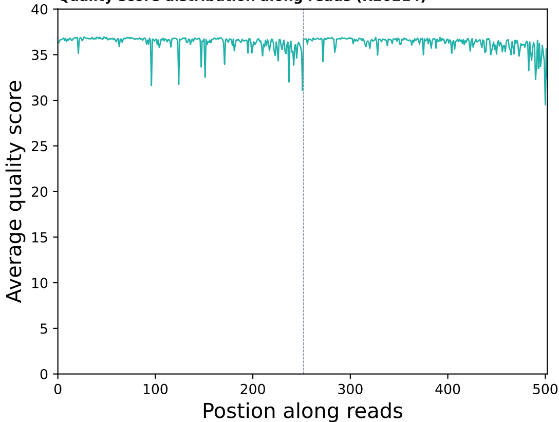
Quality score distribution along reads (R20214)
